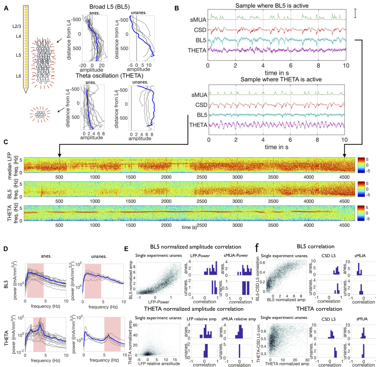
FIGURE 2 | Properties of BL5 and THETA components. (A) Spatial maps of both components across 32 channels used to record the LFP, along with diagram of putative population sources. Results for the example anesthetized experiment shown in (C) and unanesthetized experiment in Supplementary Figure 2 are highlighted in blue throughout this study. Anatomical maps indicate BL5 is made up of a larger population located within the neocortex, while THETA may be generated by a population below the neocortex. Amplitude in \text{mA}/\text{mm}^3 , distance in \mu\text{m} . (B) Segments when BL5 is active (strong low-frequency oscillations) and when THETA is active (strong sinusoidal oscillation of approximately 4 Hz). Note that the CSD and smoothed multi-unit spiking activity (sMUA) show low-frequency oscillations in both cases. Scale bar is 85th percentile amplitude of sMUA, CSD in channel 17, and ICA component taken from channel with maximum amplitude in anatomical map. (C) Spectrograms of the LFP, BL5, and THETA components for an example anesthetized experiment. (D) Average frequency spectra when BL5 and THETA are active (scaled amplitude \geq 2 ). Frequencies used to determine activity level are highlighted in pink. (E) Correlation between BL5 normalized amplitude with LFP-Power and sMUA low frequency power (1–5 Hz), and THETA normalized amplitude with LFP and sMUA relative theta amplitude. Density plot for example experiments on the left, histograms of correlation from density data on the right. (F) Correlation between BL5/THETA signal and CSD from L5 (channel 350 \mu\text{m} below L4) and sMUA. Example experiments on left, histograms of median correlations over points where BL5/THETA are active on the right.
