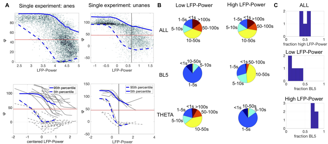
FIGURE 4 | BL5 and THETA alternate within synchronized states. (A) Top plots show density of LFP-Power vs. \phi for single experiments along with 5–95 percentile ranges. Bottom plots show ranges for all experiments with results for example experiments highlighted in blue. Anesthetized ranges are plotted against centered LFP-Power (LFP-Power minus LFP-Power with maximum range). Vertical black lines indicate median LFP-Power over unanesthetized experiments, used as the threshold between low vs. high LFP-Power. Note, by this measure all anesthetized experiments had high LFP-Power. (B) Distribution of episode lengths as a percentage of time spent in episodes of that length. (C) Fraction of time spent in each state. The top panel shows the fraction of time spent with high LFP-Power vs. low LFP-Power. The lower two panels show the fraction of time spent in BL5- vs. THETA-dominant states. Notably, approximately 30% of time in high LFP-Power is THETA-dominant. (B,C) Shows results for unanesthetized experiments only.
