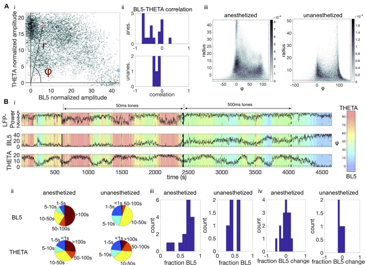
FIGURE 3 | BL5 and THETA alternate within experiments. (A,i) Density plot of BL5 vs. THETA normalized amplitude for an example anesthetized experiment (same as Figure 1B ). Pink and blue marks indicate points that are used for example BL5 and THETA active segments in Figure 1B , respectively. We set \phi as the angle from the BL5-axis, while r is the radius. (ii) Correlations of BL5 vs. THETA normalized amplitude for each experiment. (iii) Conglomerate density plots of \phi vs. radius for all anesthetized and unanesthetized experiments. (B,i) Time course of \phi over the same example anesthetized experiment used in Figure 1 . (ii) Pie charts showing the amount of time spent in BL5- vs. THETA-dominant episodes. For example, for anesthetized experiments during THETA-dominant states about 1/3 of time spent is in an episode of length 10–50 s. (iii) Histogram of the fraction of time spent in BL5- vs. THETA-dominant states. (iv) Histograms of the difference in fraction of time dedicated to BL5-dominant states during tone presentations vs. spontaneous activity.
