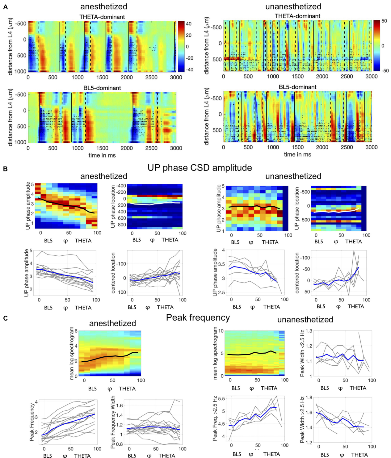
FIGURE 6 | Neocortical activity differs depending on BL5- vs. THETA-dominant states. (A) CSD (color, \text{mA}/\text{mm}^3 ) and spiking activity (black asterisks) from example anesthetized and unanesthetized experiments seen in previous figures. UP state onsets are marked by solid black lines, while DOWN state onsets are marked by dashed lines. (B) Top plot shows density of UP state amplitude and UP state amplitude peak location for individual experiments, along with the mean with respect to \phi . Density is normalized for each \phi bin, and the mean for a \phi bin is calculated only if there are \geq 30 points. We only included synchronized data points. Lower plots show the mean for all experiments, with highlighted results for the example experiment above. UP peak location is centered along the mean location for each experiment (UP location minus UP location mean). (C) Top left plot shows average spectrogram values over \phi for the same example experiments as above, along with the mean peak frequency over \phi . Other plots show means for all experiments, with highlighted results for the example experiment.
